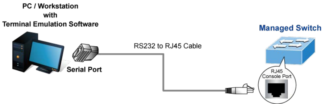
Figure 2-1 Industrial Managed Switch Console Connectivity
